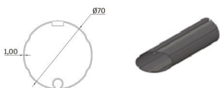
1 Roller Tube Ø70
