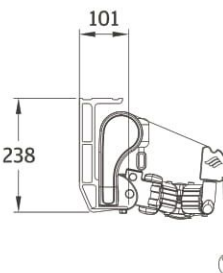
Ceiling Installation Bracket
