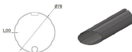
2 Roller Tube Ø78
