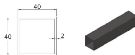
3 Iron Profile 40x40
