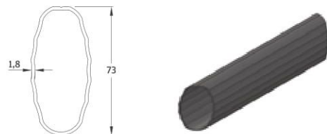
6 Arm Profile
