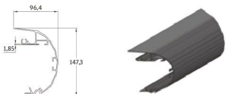
7 Front Profile
