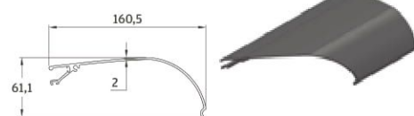
6 Arm Profile
