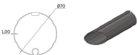
1 Roller Tube \varnothing 70
