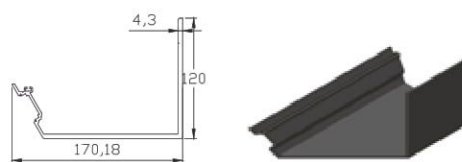
2 Side and Front Gutter Profile
