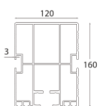
1 Rafter Profile
