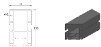
1 Rafter Profile
